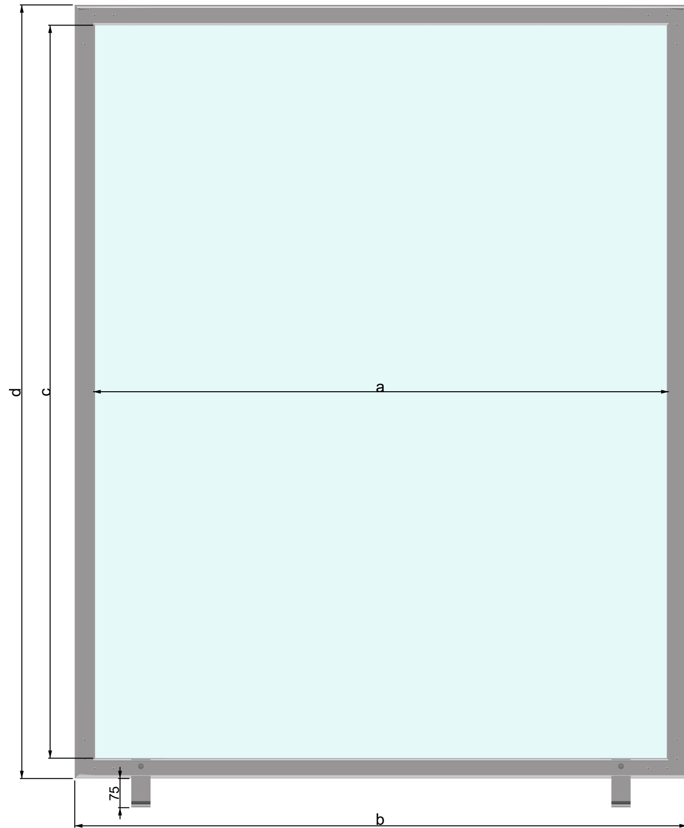
Front view [1:10]
